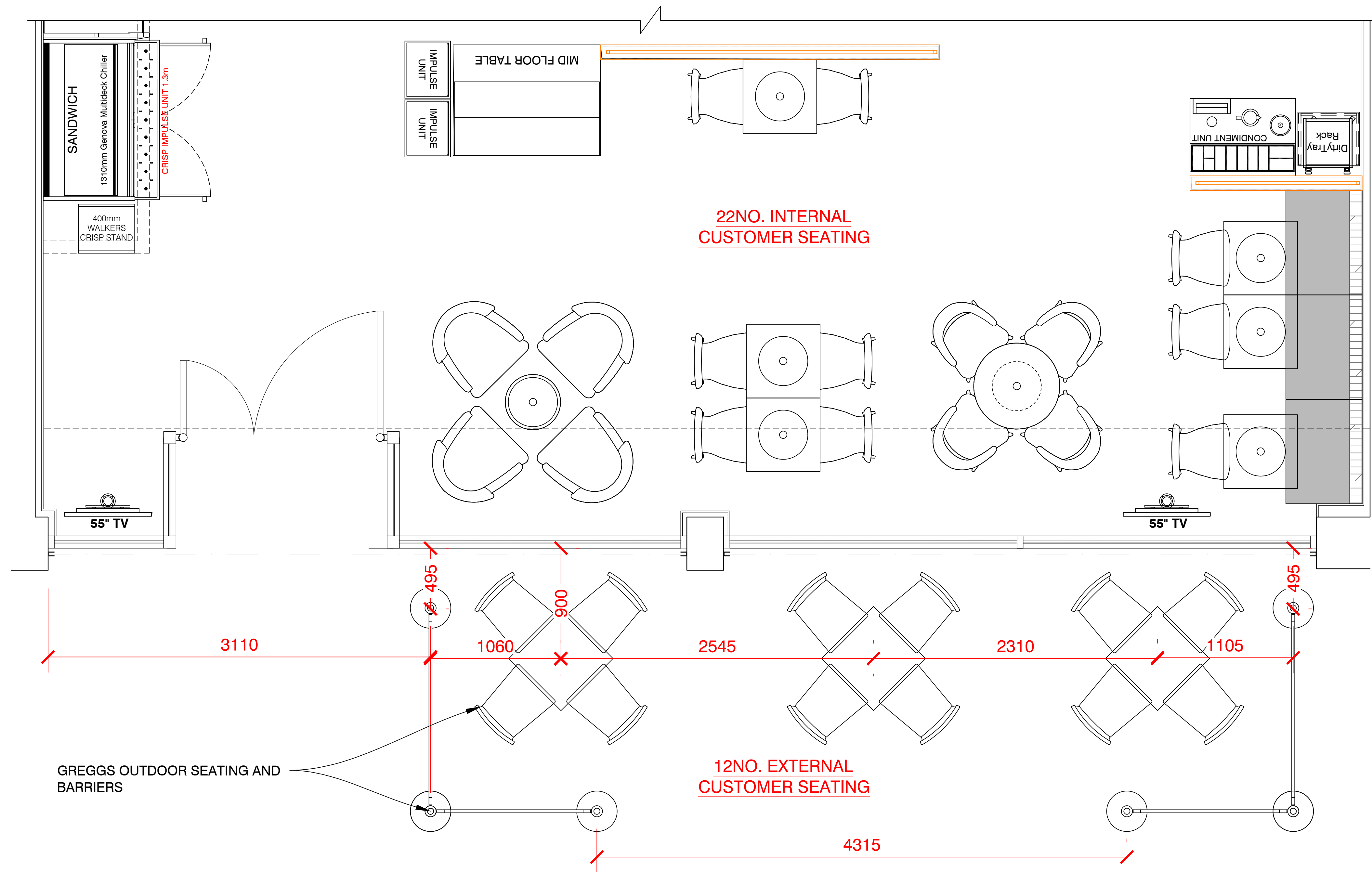
PROPOSED EXTERNAL SEATING (1:20)
