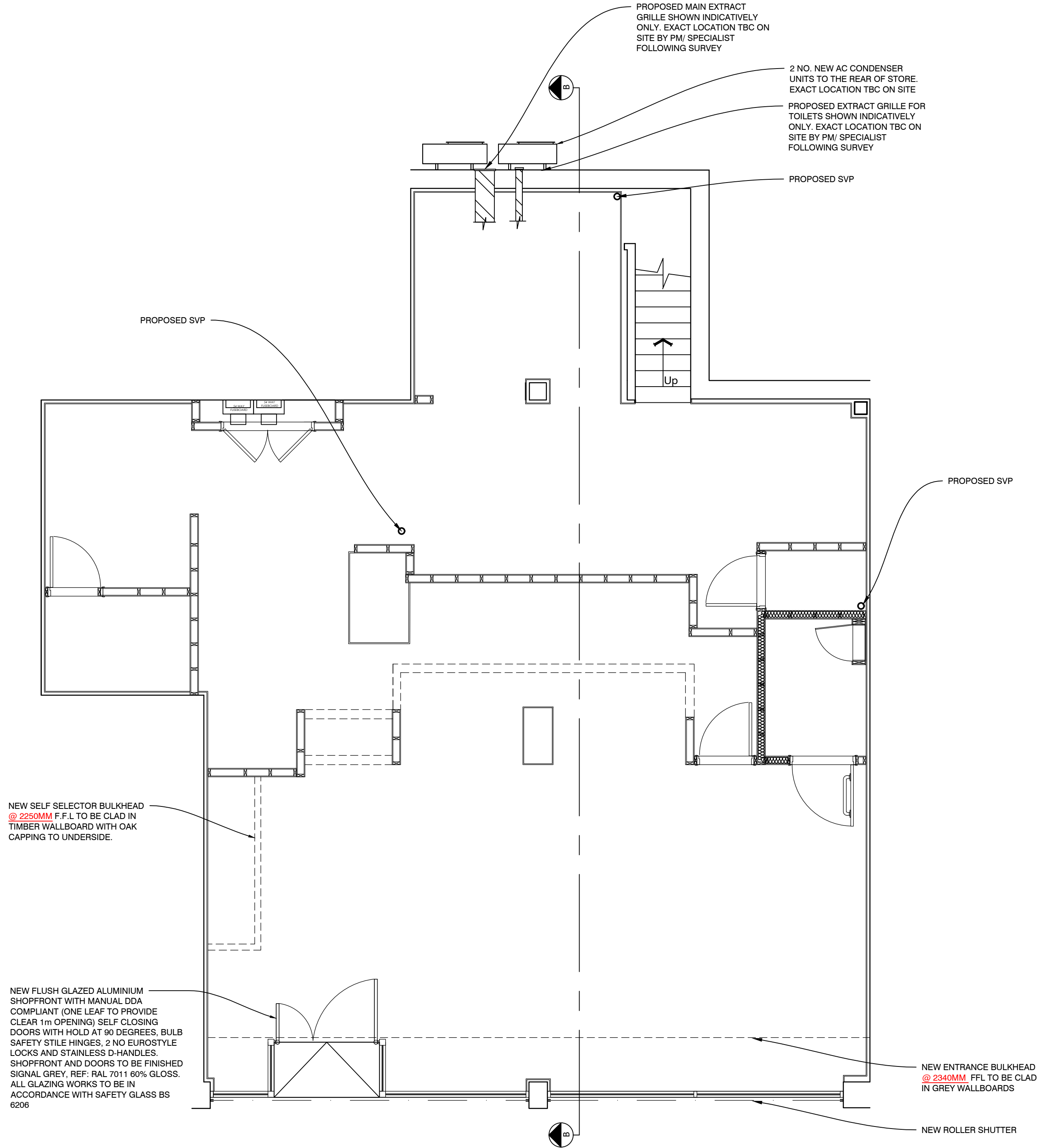
PROPOSED GA PLAN (1:50)
