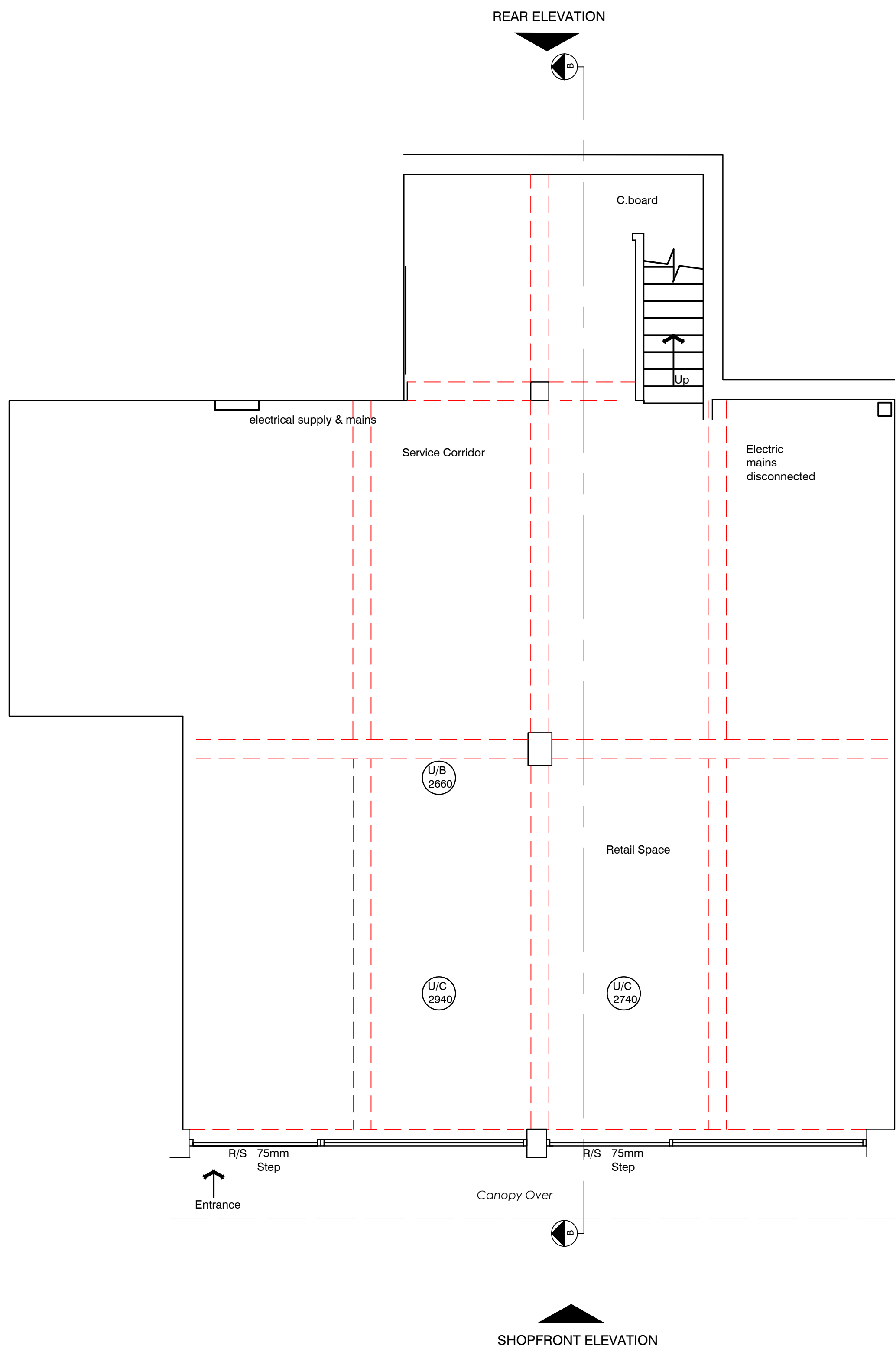
EXISTING GA PLAN - GROUND FLOOR (1:50)
