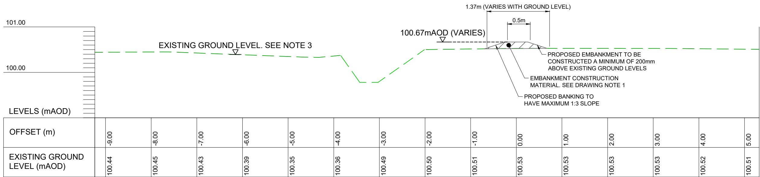
SECTION L-L
