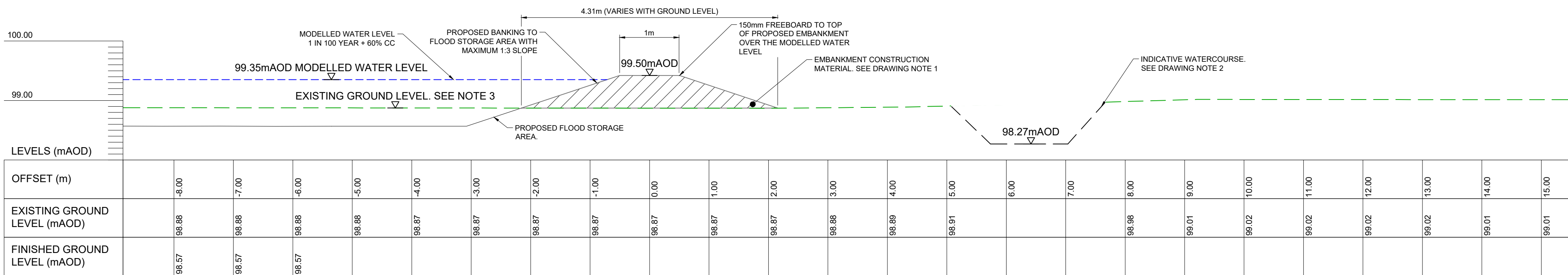
SECTION C-C
