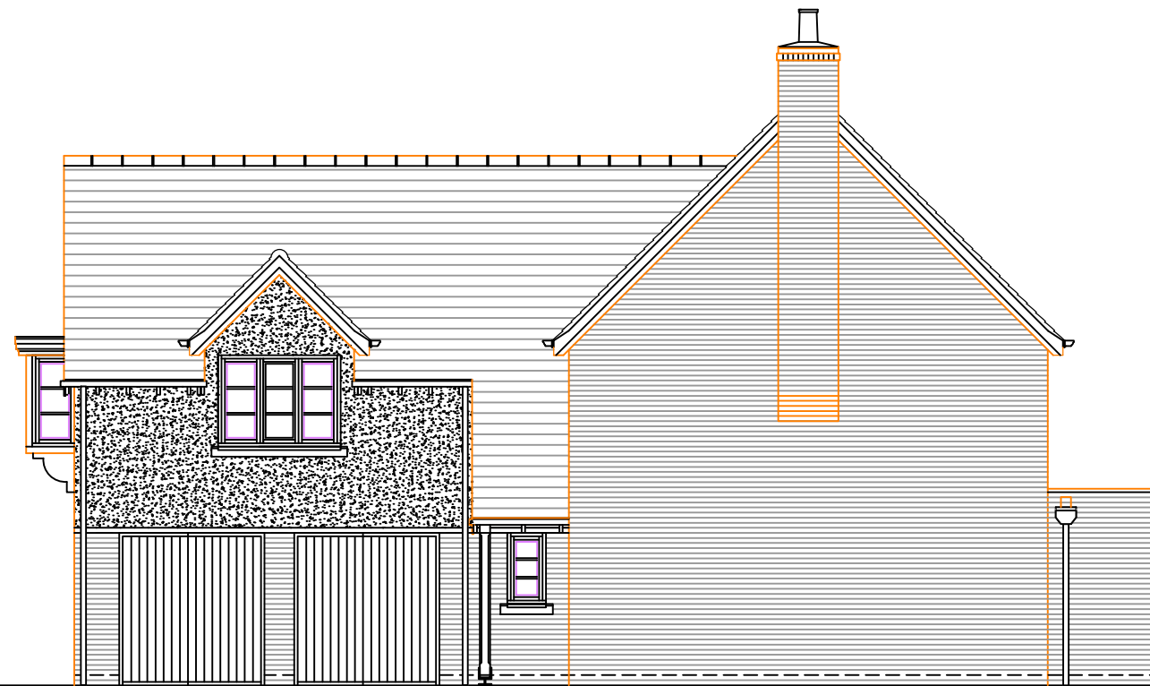
SIDE ELEVATION
