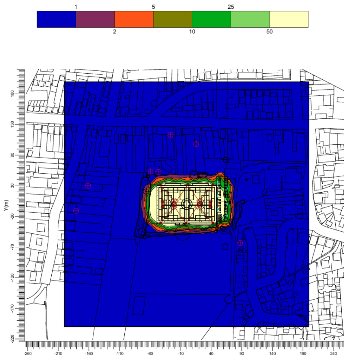
Figure 3 – Spillage for the proposed AGP (Lux)
