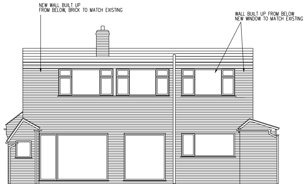
REAR ELEVATION PROPOSED
