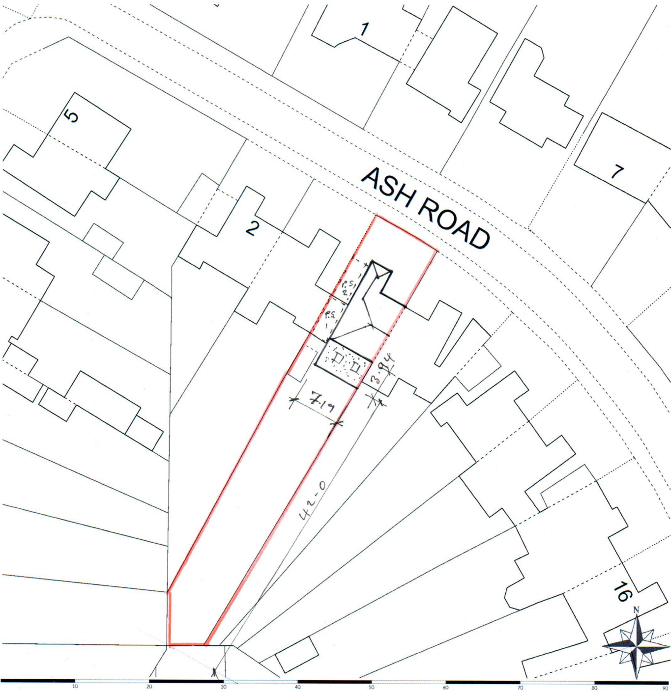
Scale: 1:500 | Area < 1Ha | Grid Reference: 445953,297129 | Paper Size: A4
