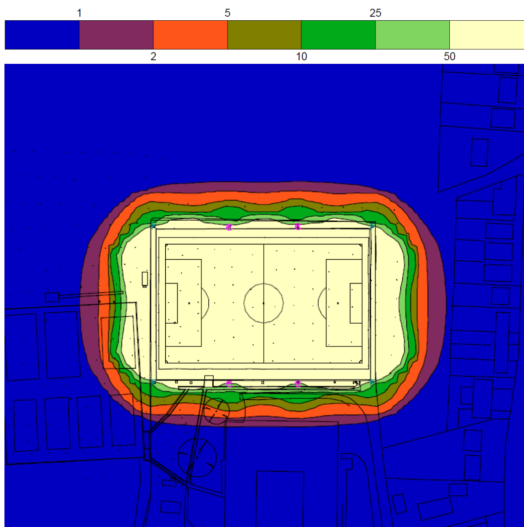
Figure 3 – Spillage for the proposed AGP (Lux)
