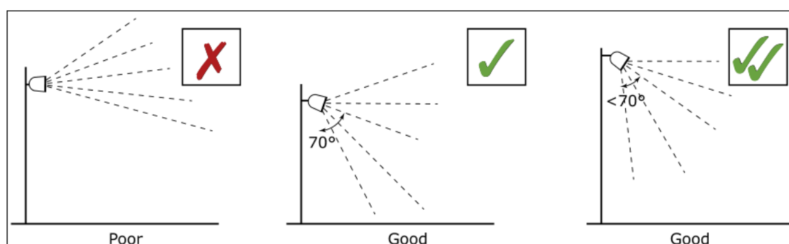
Figure 5 – Light angle tilt to not contribute to sky glow
