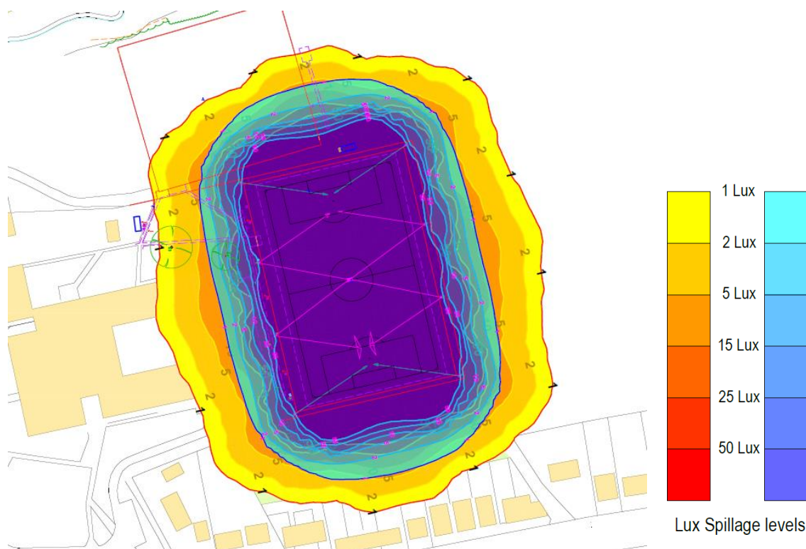
Figure 4 – Spillage Comparison
