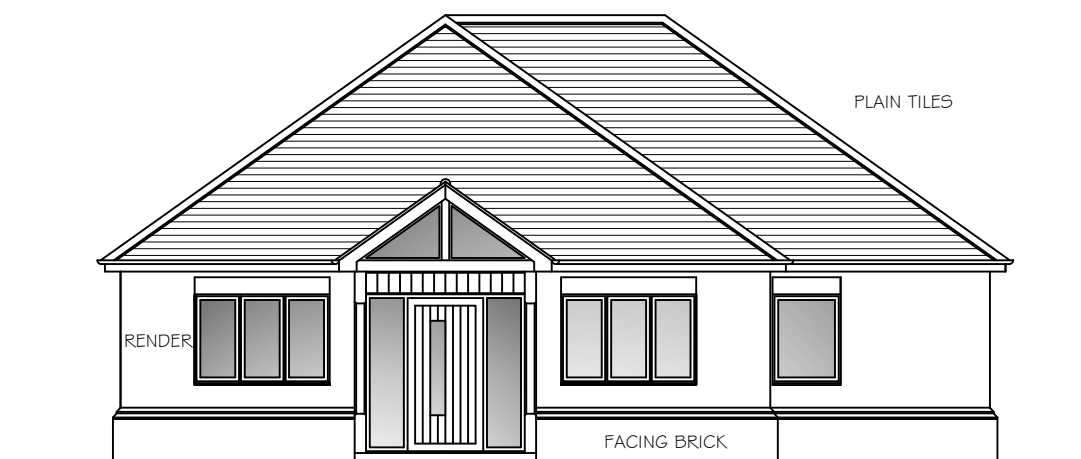
FRONT
