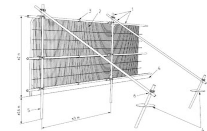
BS5837 Default tree protection barrier specification
