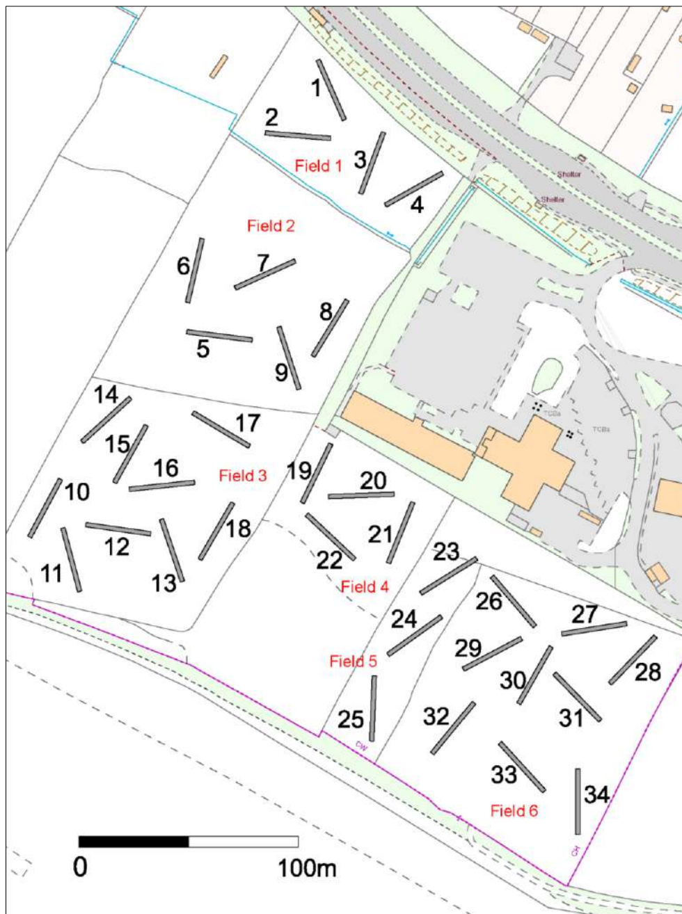
Figure 3: Trench plan across the proposed development area
