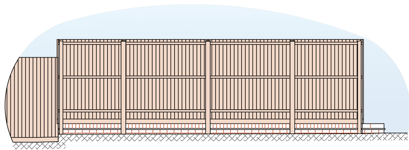
EXISTING ELEVATION A (SCALE 1:50)
