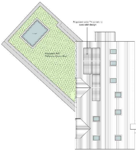
Roof Plan
