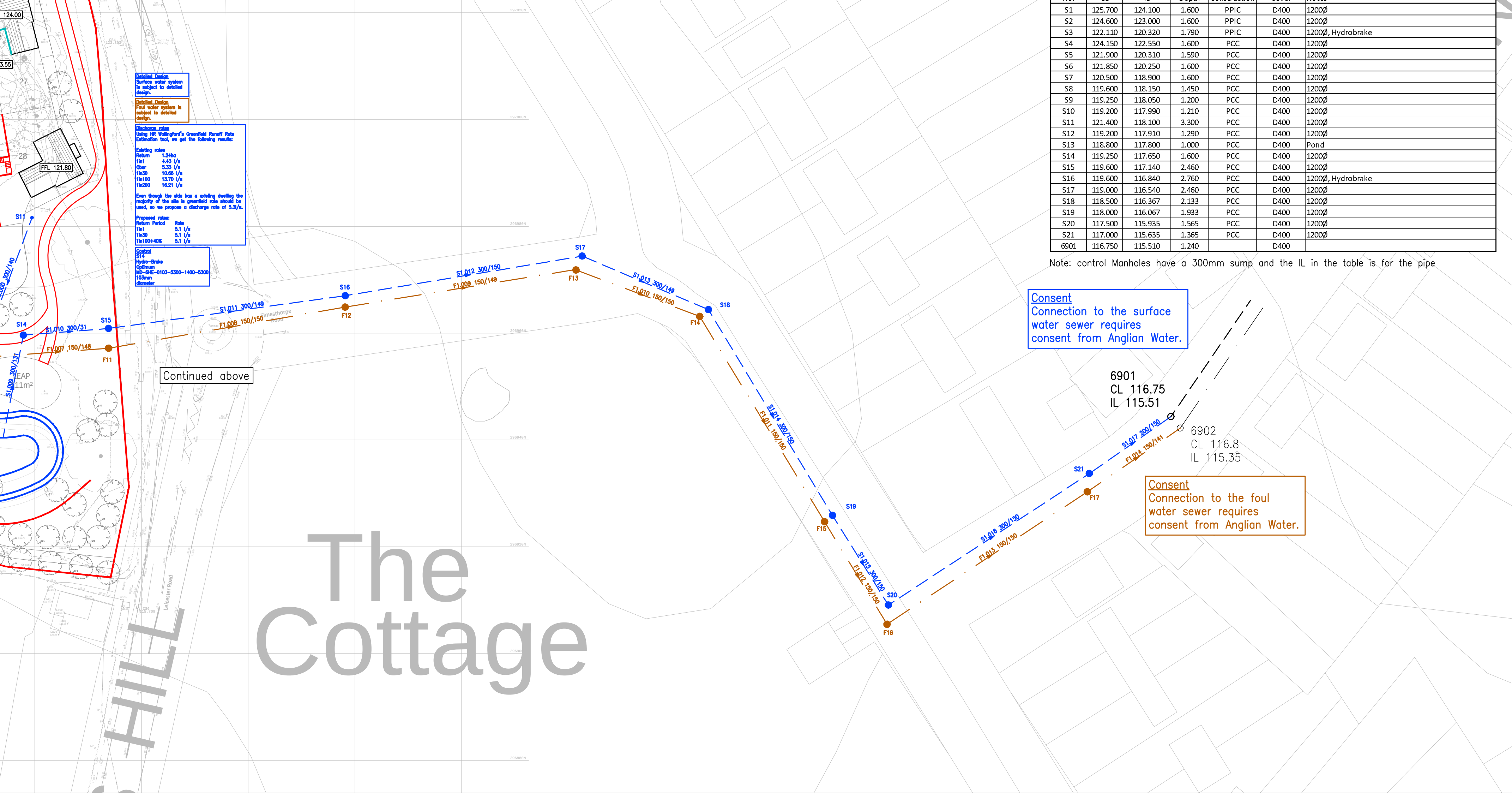
Foul Water Pipeline Schedule
