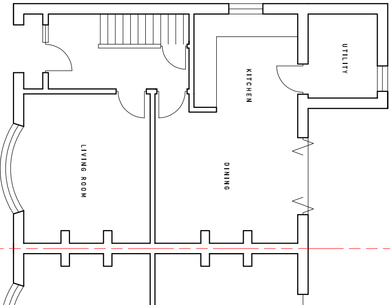
EXISTING GF PLAN
