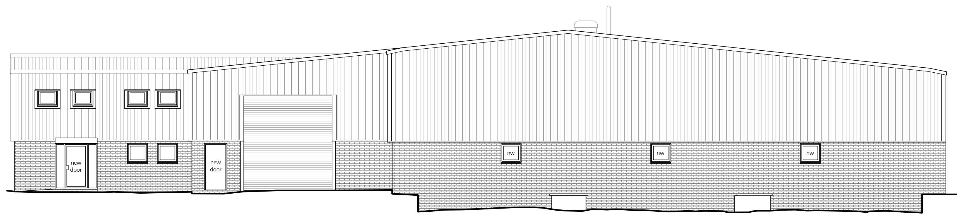
elevation : south east : as proposed
