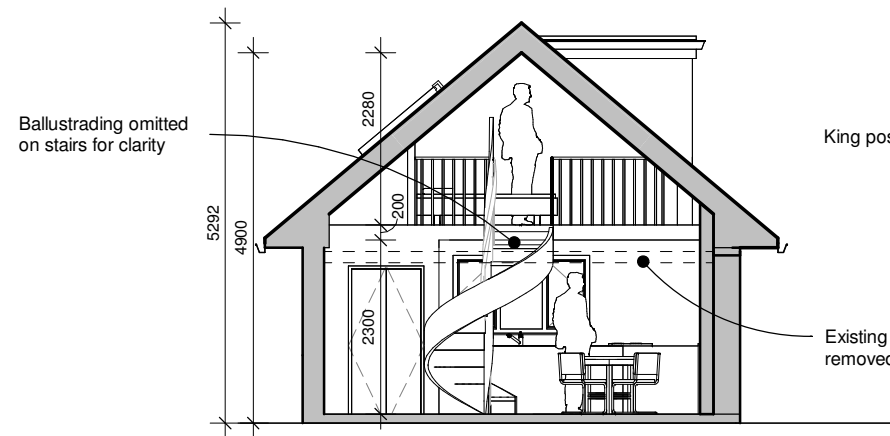
Section
