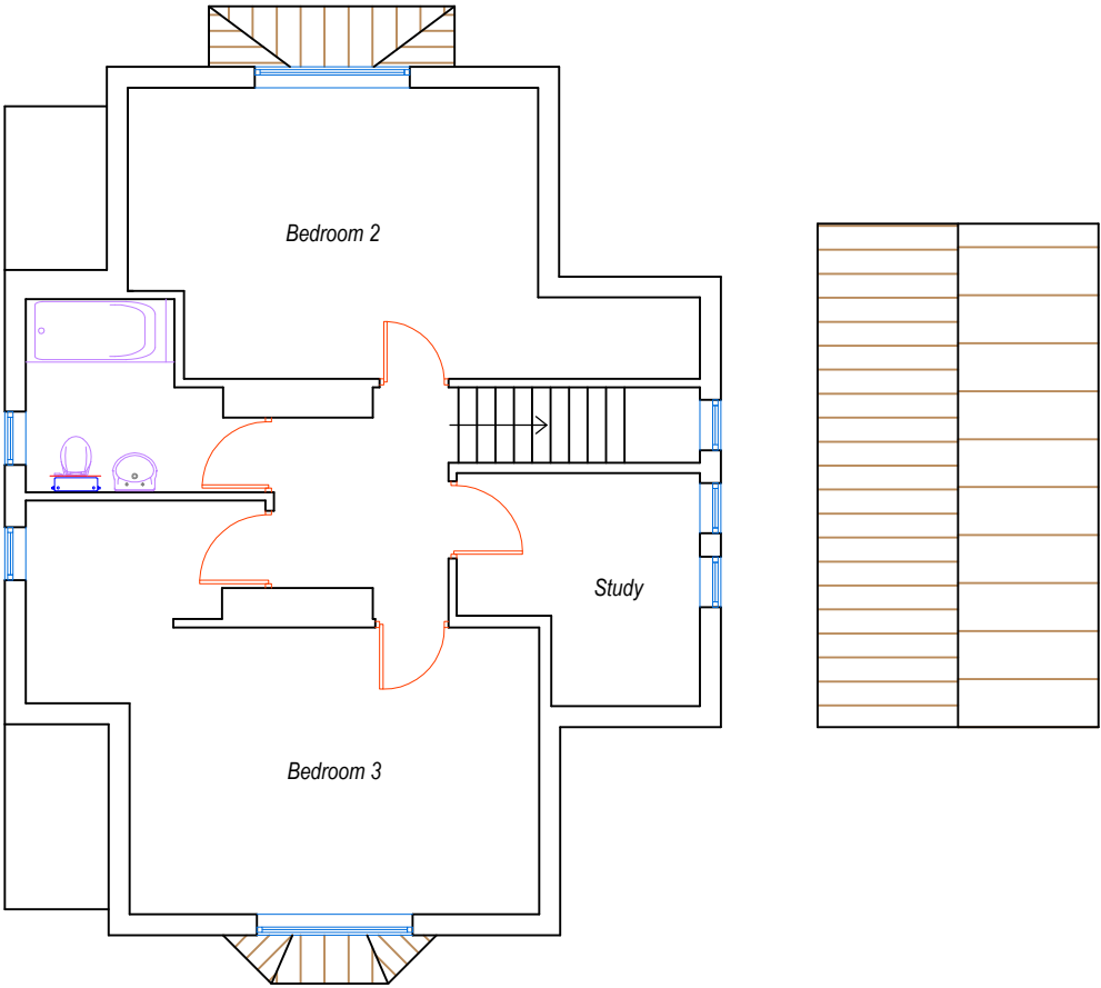
Existing First Floor Plan @ 1:100 (A3)
