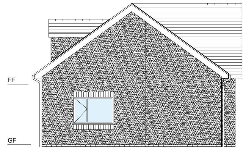
East elevation.
