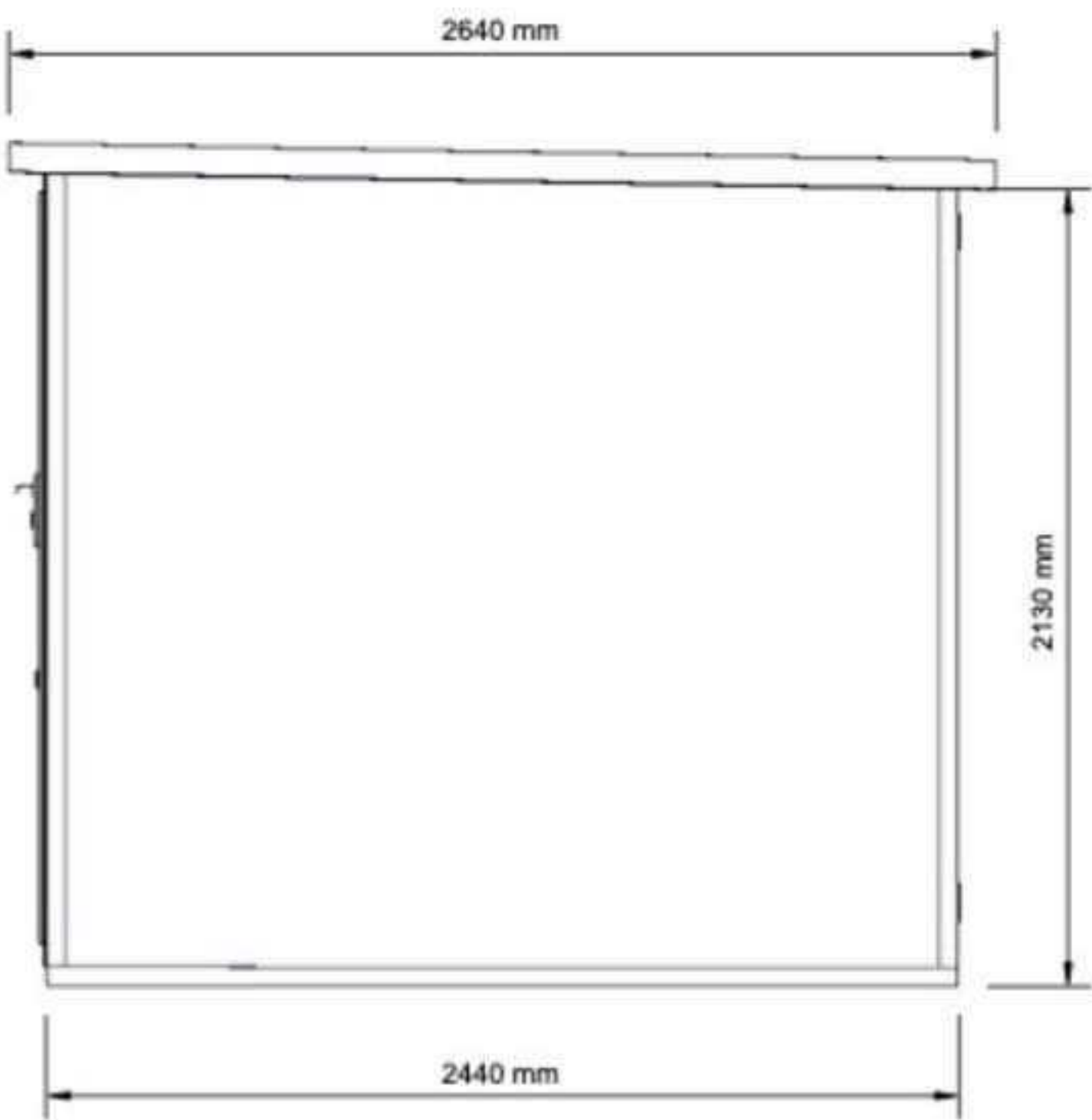
RIGHTHAND ELEVATION
