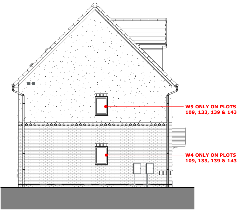
LEFT ELEVATION
