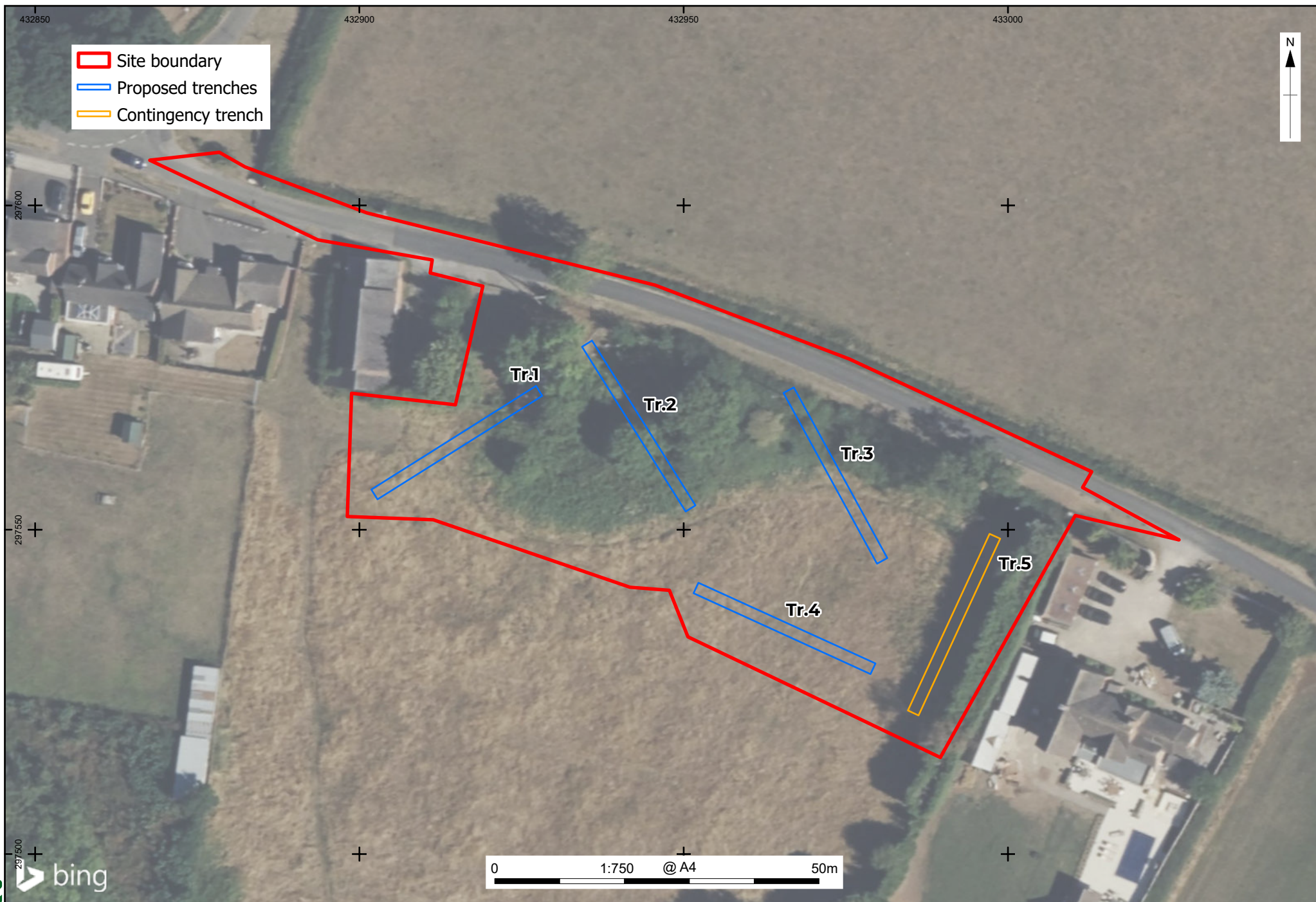
Figure 2: Proposed trench locations
