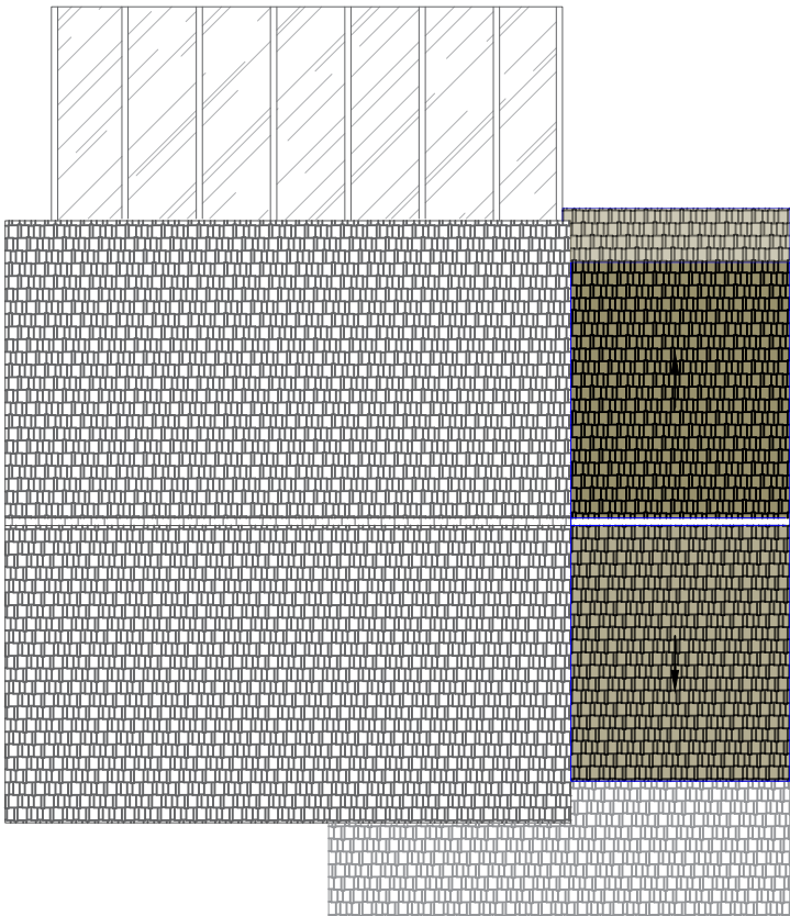
PROPOSED ROOF PLAN 1:100 AT A3
