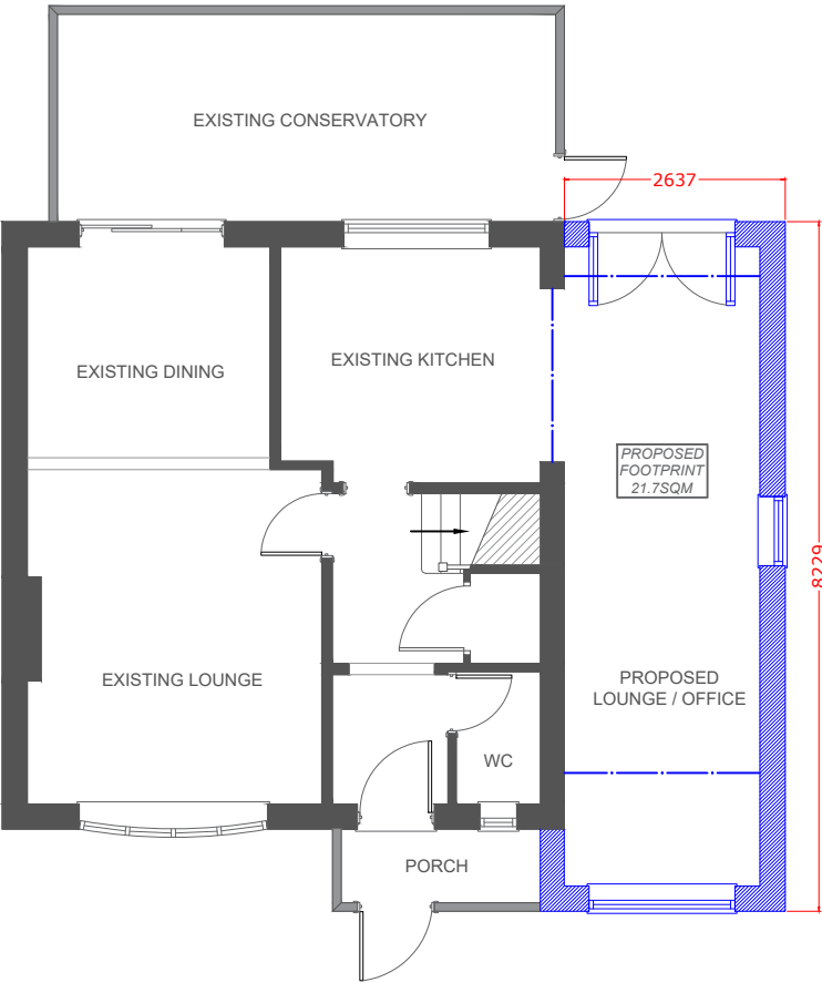
PROPOSED GF PLAN 1:100 AT A3
