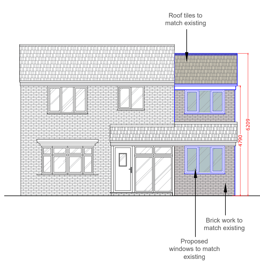
PROPOSED FRONT ELEVATION 1:100 AT A3
