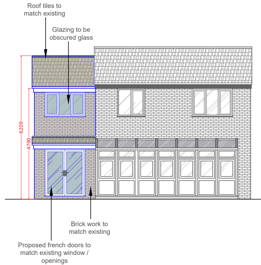
PROPOSED REAR ELEVATION 1:100 AT A3
