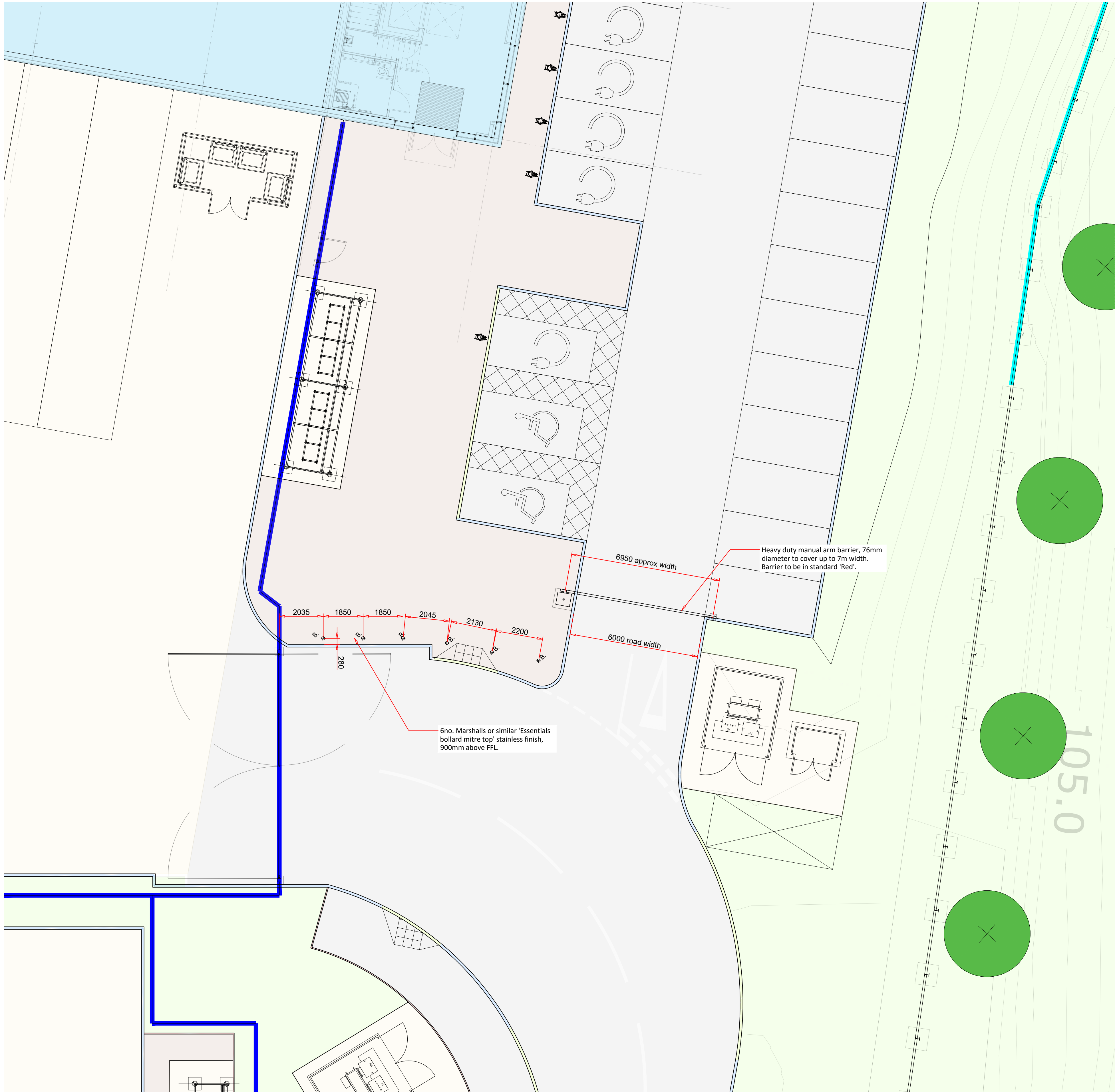
Unit 3 Entrance Sketch Scale 1:100 @ A1
