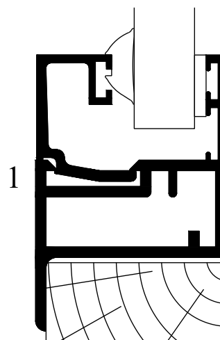
SERIES 40 11.5mm SQUARE BEAD OPTION
