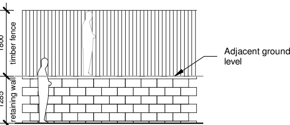
Retaining wall with fence over. Worst case scenario = 1285mm retaining wall between plots 1 & 2
