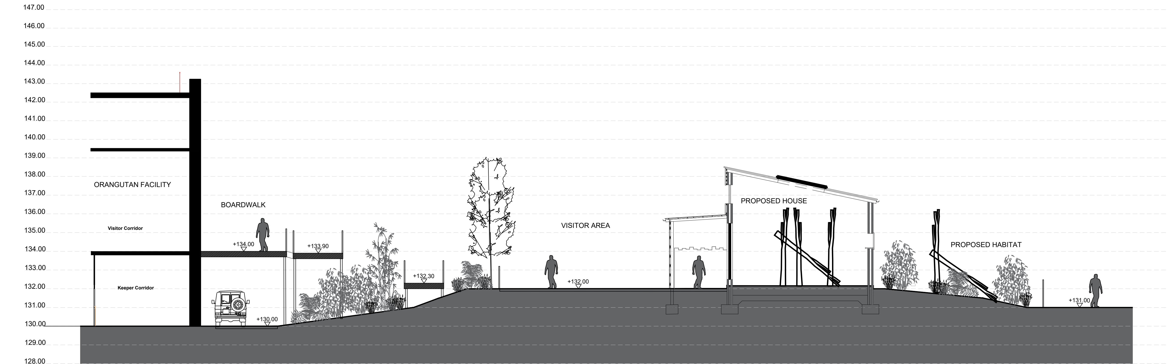
SITE SECTION 08: THROUGH ORANGUTAN FACILITY AND PROPOSED ANIMAL HOUSE
