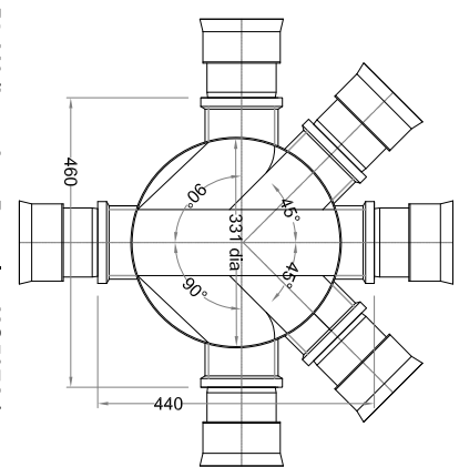
PLAN (based on Polypipe UG537A)
