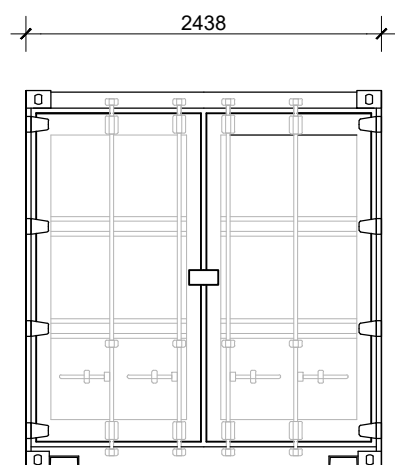
Front View(Door)
