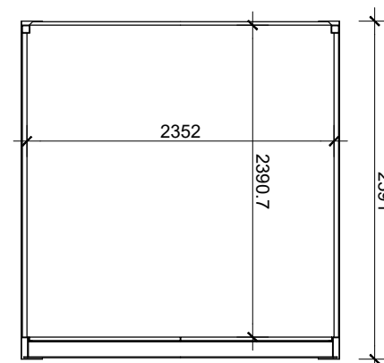
Cross Section
