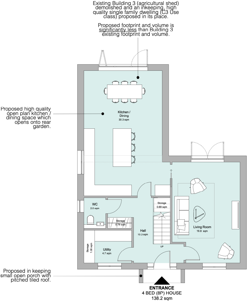
1 proposed ground floor
