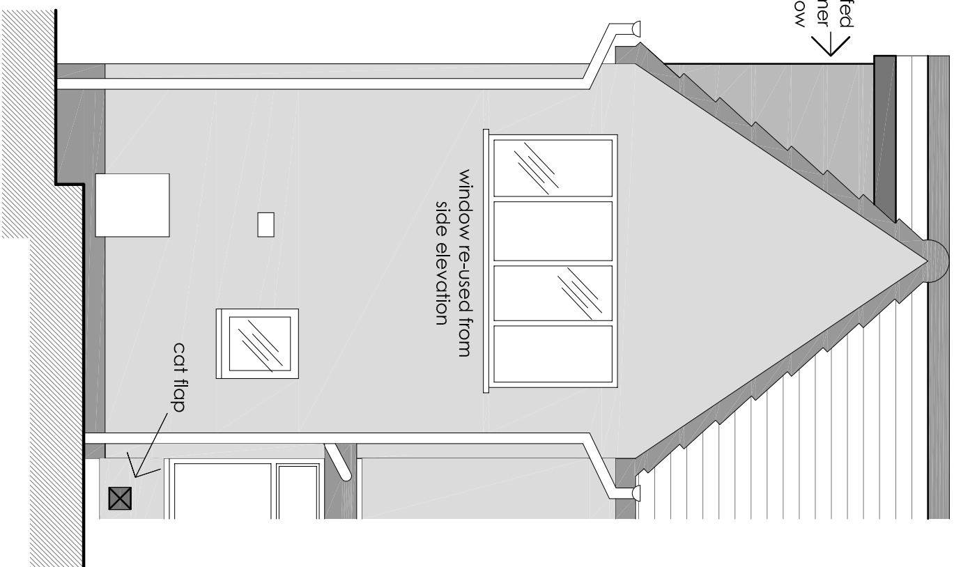
Proposed Rear Elevation (East Facing)
