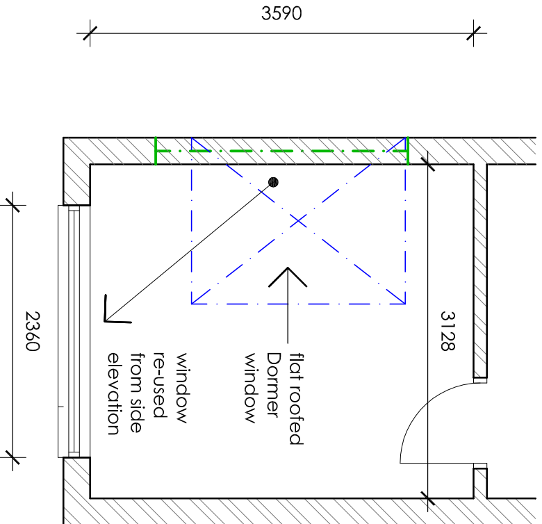
Proposed Floor Plan of Bedroom
