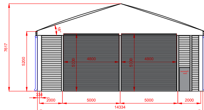
Elevation D
