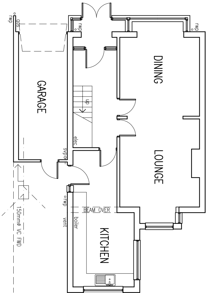
GROUND FLOOR PLAN (GIA 70.5m 2 )
