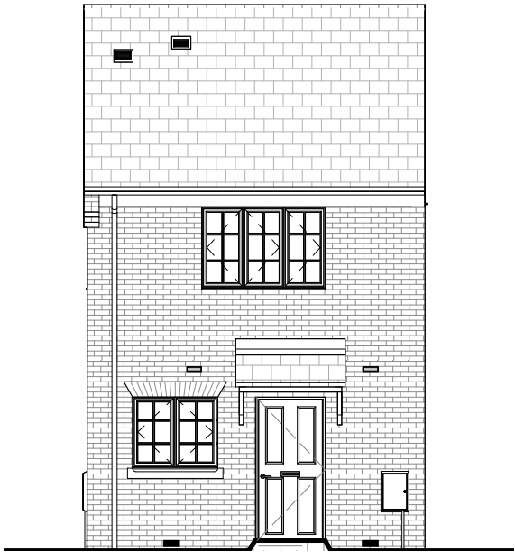
Front Elevation
