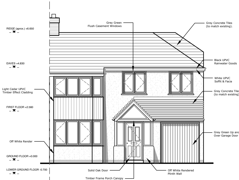
Elevation A (North)
