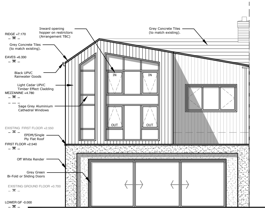
Elevation C (South)
