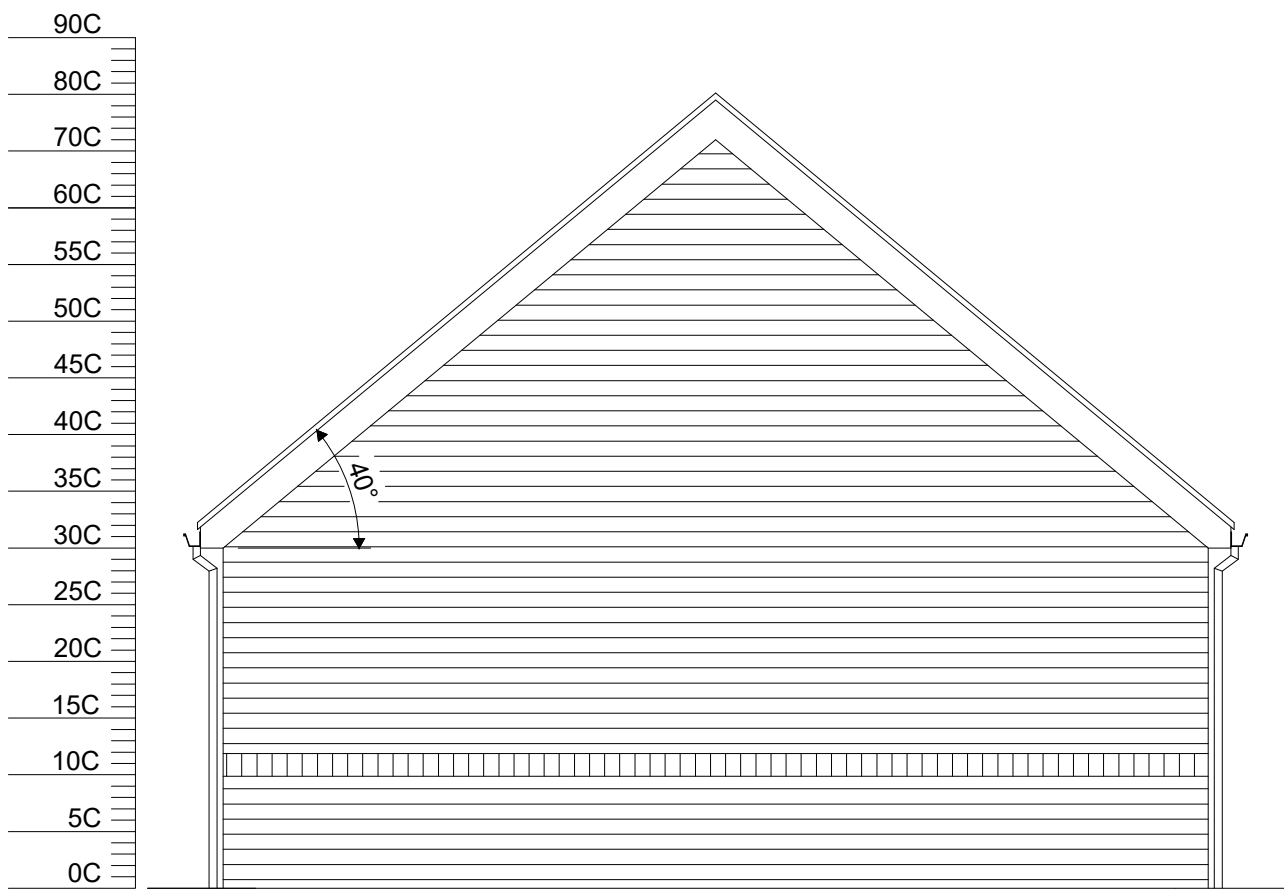
REAR ELEVATION
