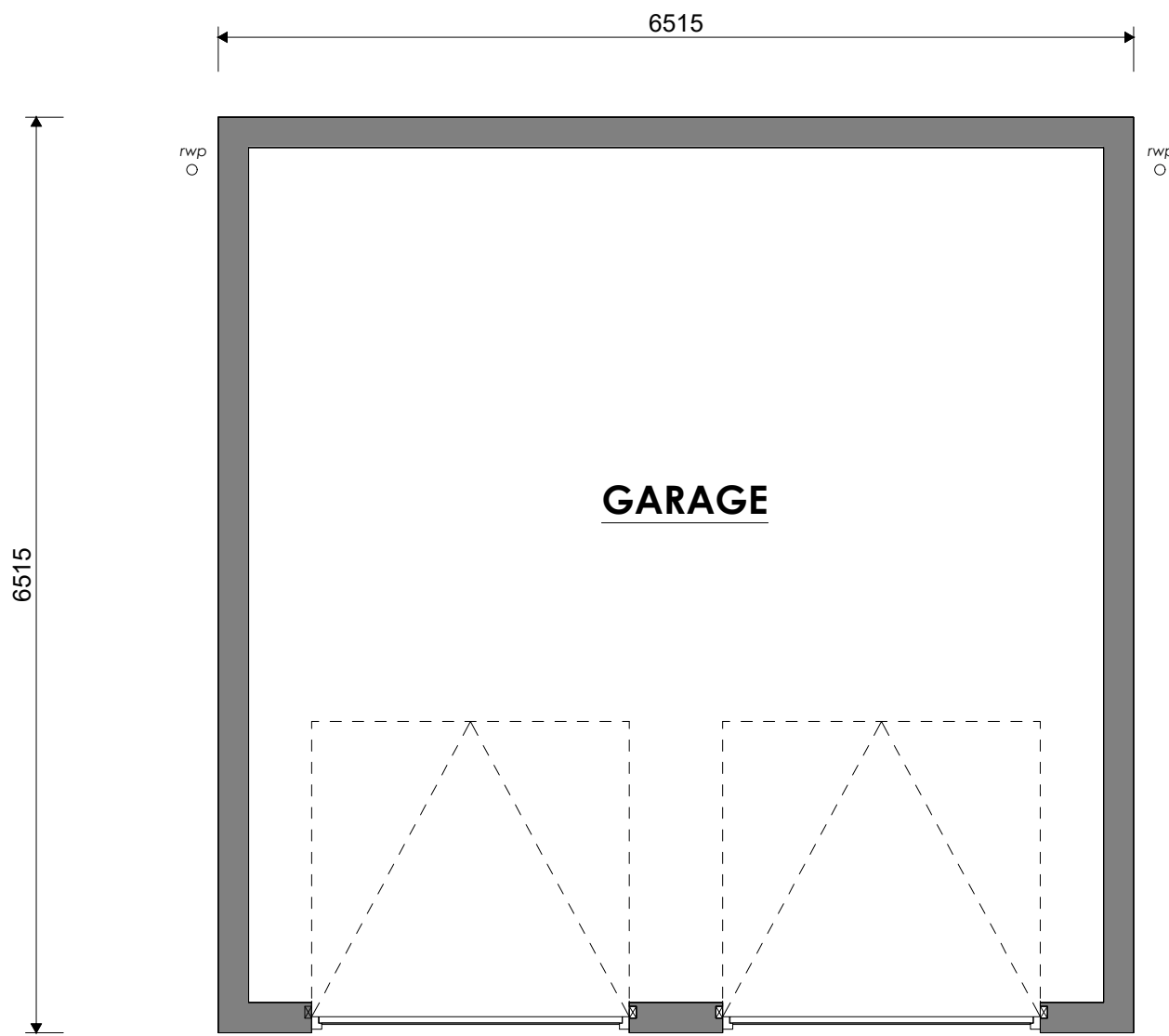
FLOOR PLAN
