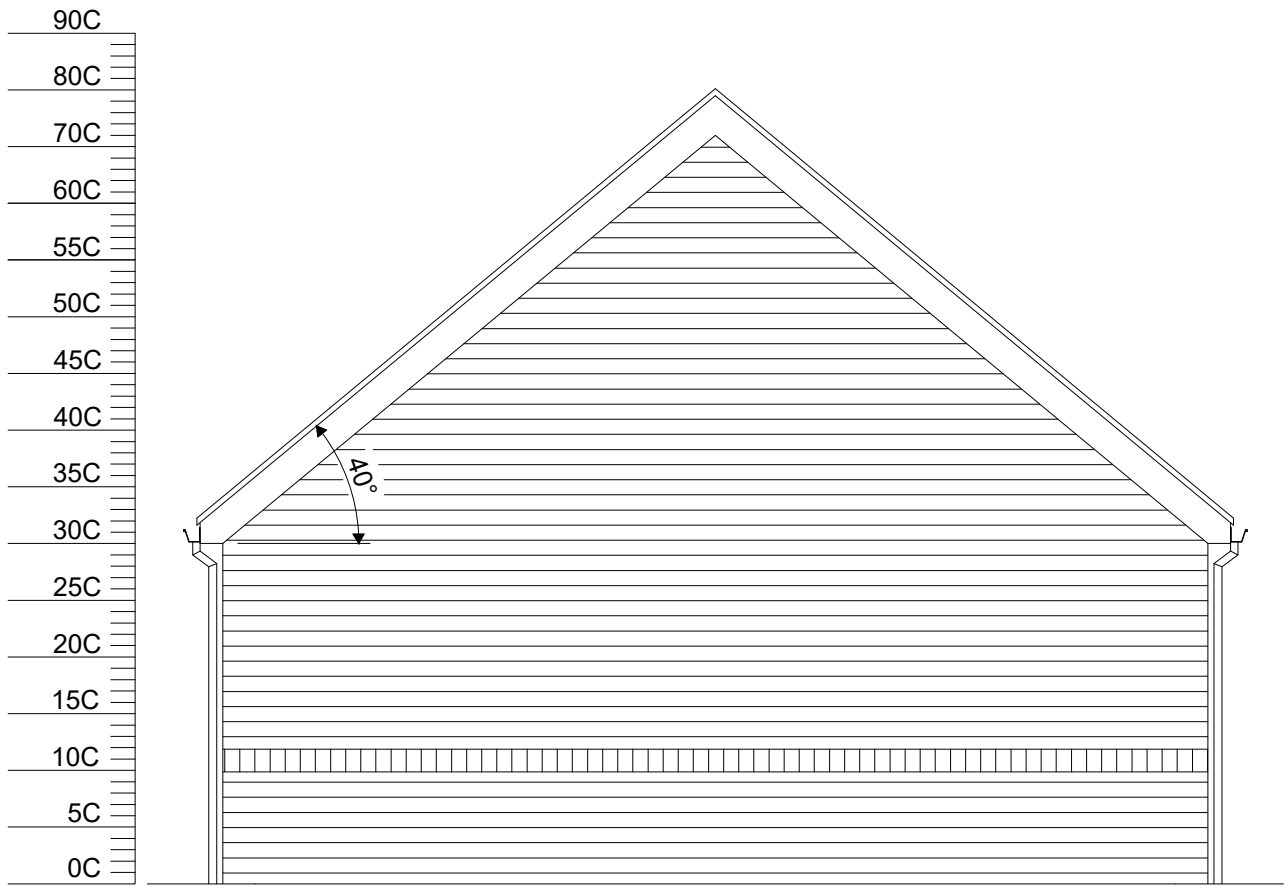
SIDE ELEVATION 1
