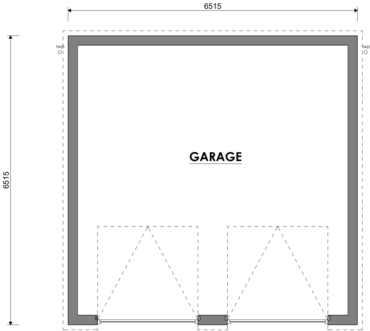
FLOOR PLAN
