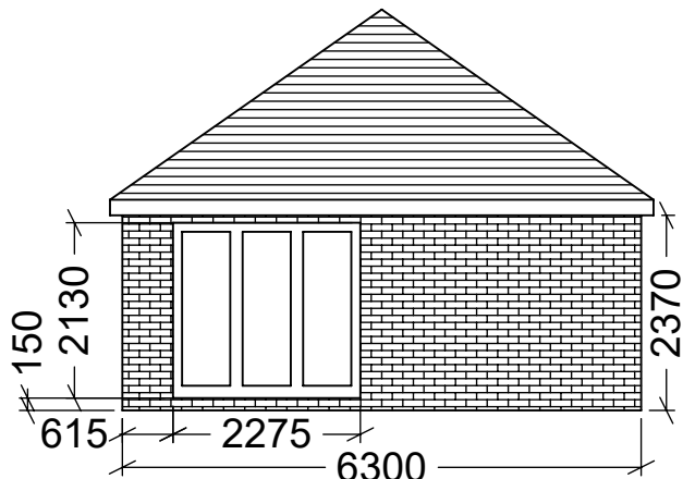
Side NW Facing Bifold door as seen from garden PROPOSED
