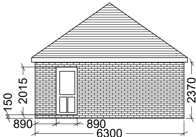
Side NW Facing Personnel door as seen from garden
