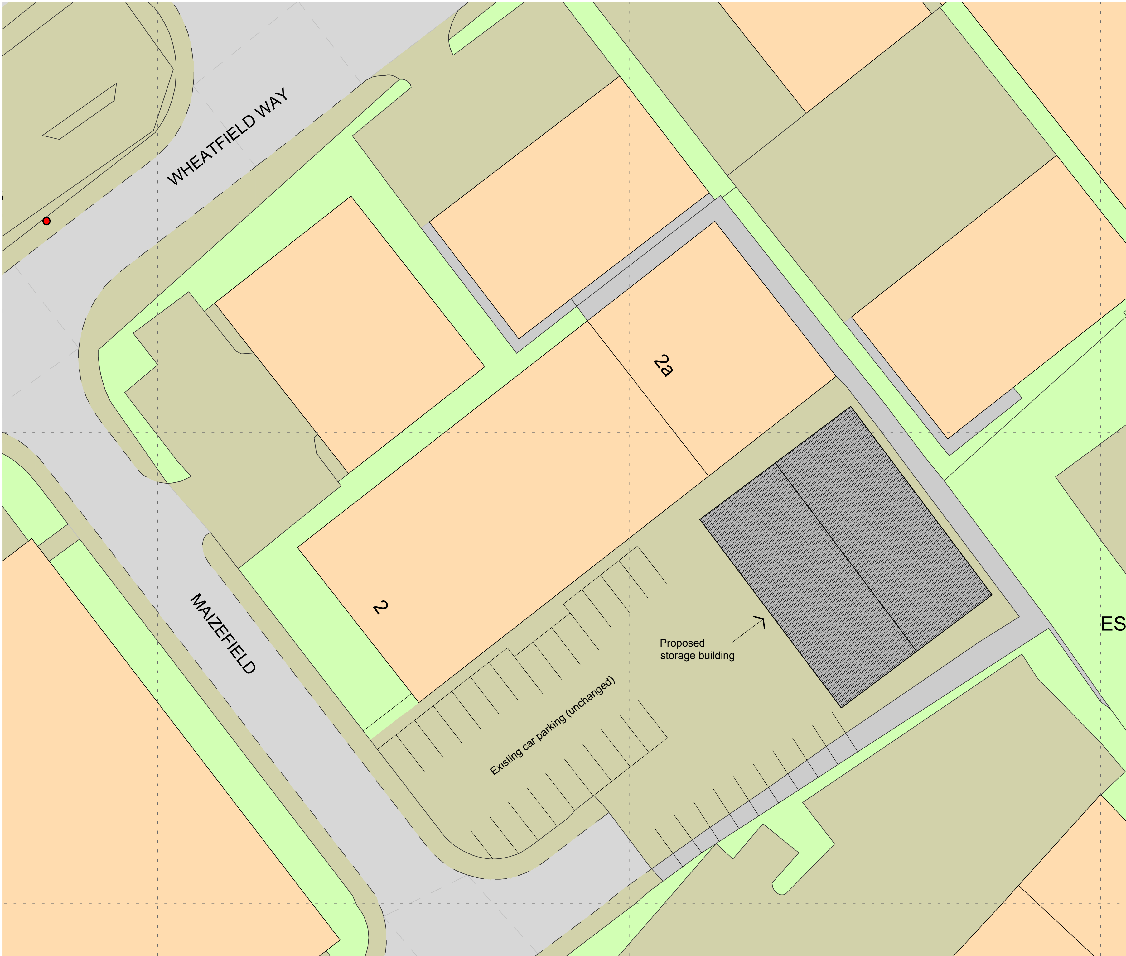
Proposed Block Plan (1:250)
