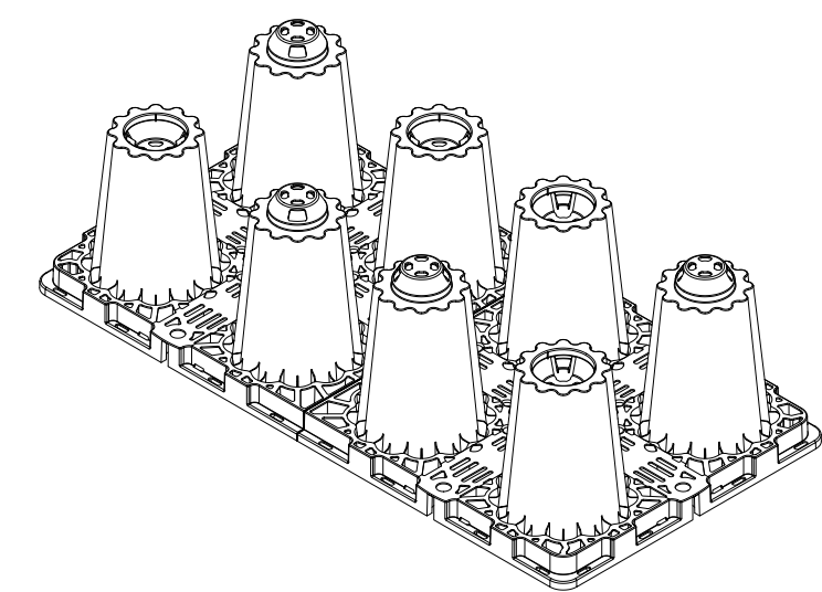
Isometric view of Single ACO StormBrixx HD System Unit
