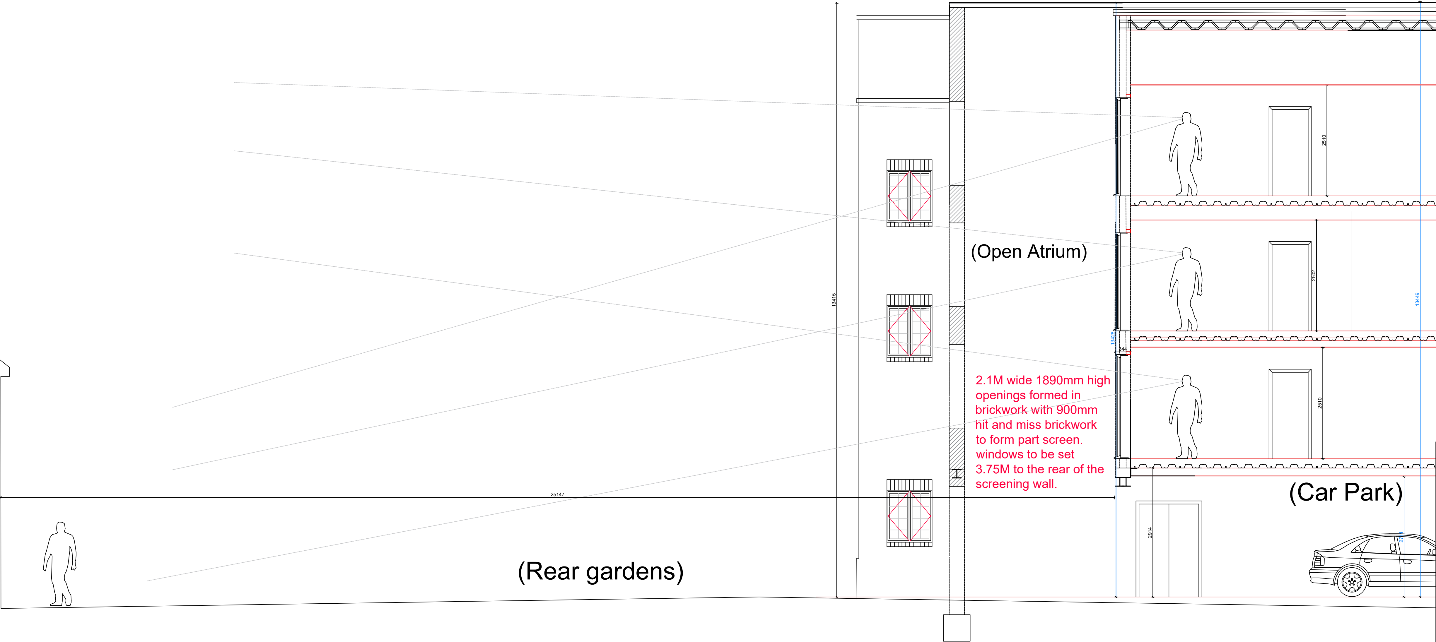
Proposed Section through Atrium( From T
