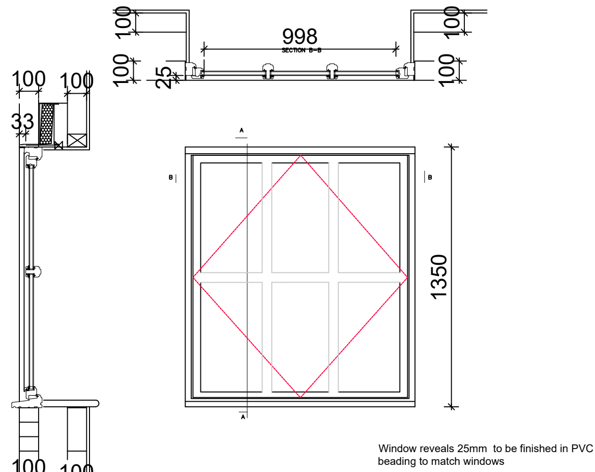
Standard Casement Window Sections
