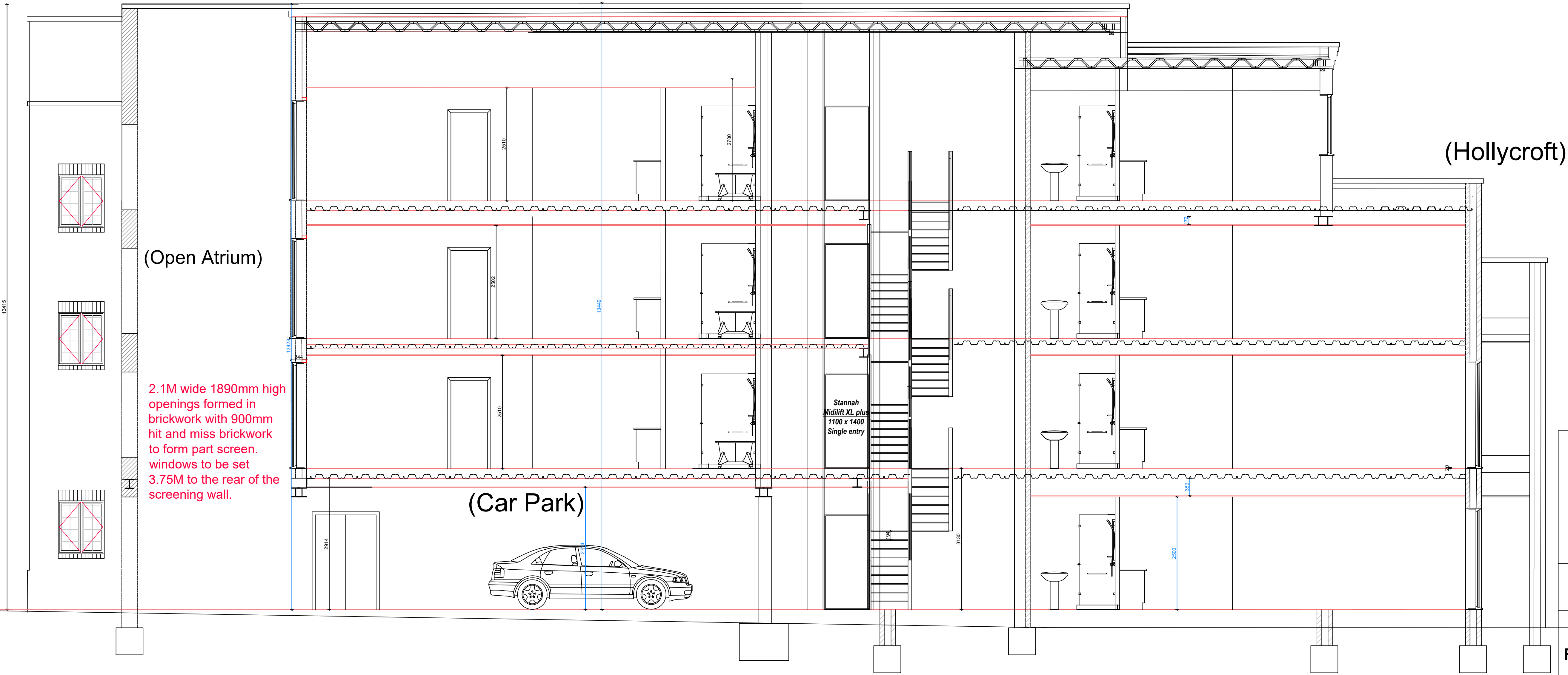
Proposed Section through Atrium( From Trinity Lane)
