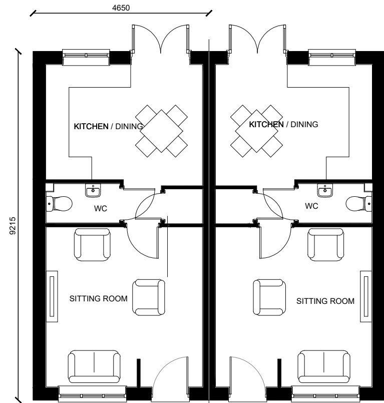
PROPOSED GROUND FLOOR PLAN AS OPP
