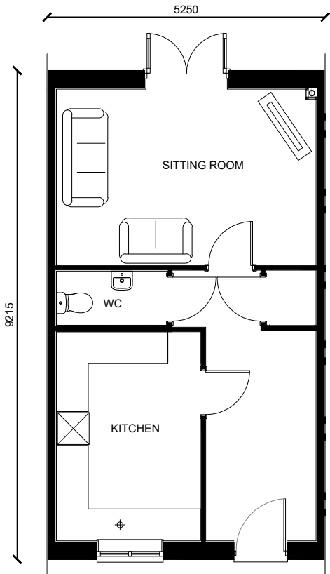
PROPOSED GROUND FLOOR PLAN AS
