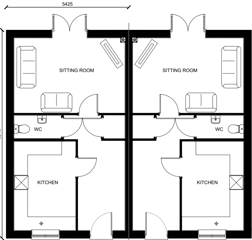
PROPOSED GROUND FLOOR PLAN AS
